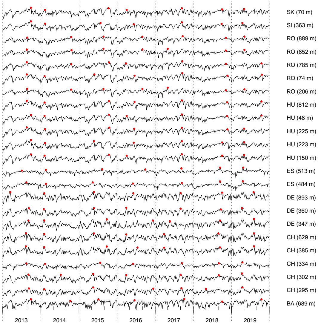
FIGURE 2. Daily temperature maxima (solid black curves) for the months of June, July and August during the period 2013–2019 at the 23 stations with the most complete records. Annual temperature maxima are indicated by red dots. The corresponding country code (in alphabetical order from bottom to top) and elevation of each station are provided on the right-hand side. In our data analysis, we used only the annual maxima until 2018 for fitting, and left the 2019 maximum out for risk assessment.
