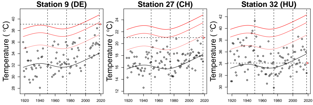
FIGURE 6. Plot of observed annual maxima (dots), estimated time trend (solid black), and estimated 10, 100 and 1000 year-return level curves (from light to dark red) for 3 selected stations located in Germany, Switzerland and Hungary (left to right). The red dot in each panel represents the observed annual maximum for 2019 (not used to fit the model). The four vertical dashed lines correspond to the reference years of 1950, 1975, 2000, and 2018.
