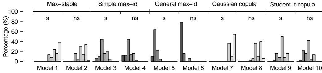
FIGURE 7. Logarithmic score (15) ranks computed for 50 bootstrap simulations from the fitted Model 6, for each of the 10 models. The bars show the percentage of ranks ranging from 1 (best score) to 10 (worst score) for each of the Models 1–10, with darker grey (towards the left side of each histogram) indicating better rank. The letter “s” means “stationary”, whereas “ns” means “non-stationary”.
