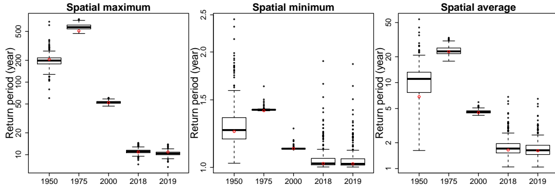
FIGURE 12. Boxplots of bootstrapped return periods (on logarithmic scale) of the 2019 annual maximum, computed for the spatial maximum, minimum and average (left to right) over 31 stations, based on 10^5 random fields simulated from our best non-stationary spatial Model 6 (fitted to the annual maxima for the period 1918–2018), with respect to 1950, 1975, 2000, 2018 and 2019 as reference years. Red dots are pointwise estimates of these return periods.
