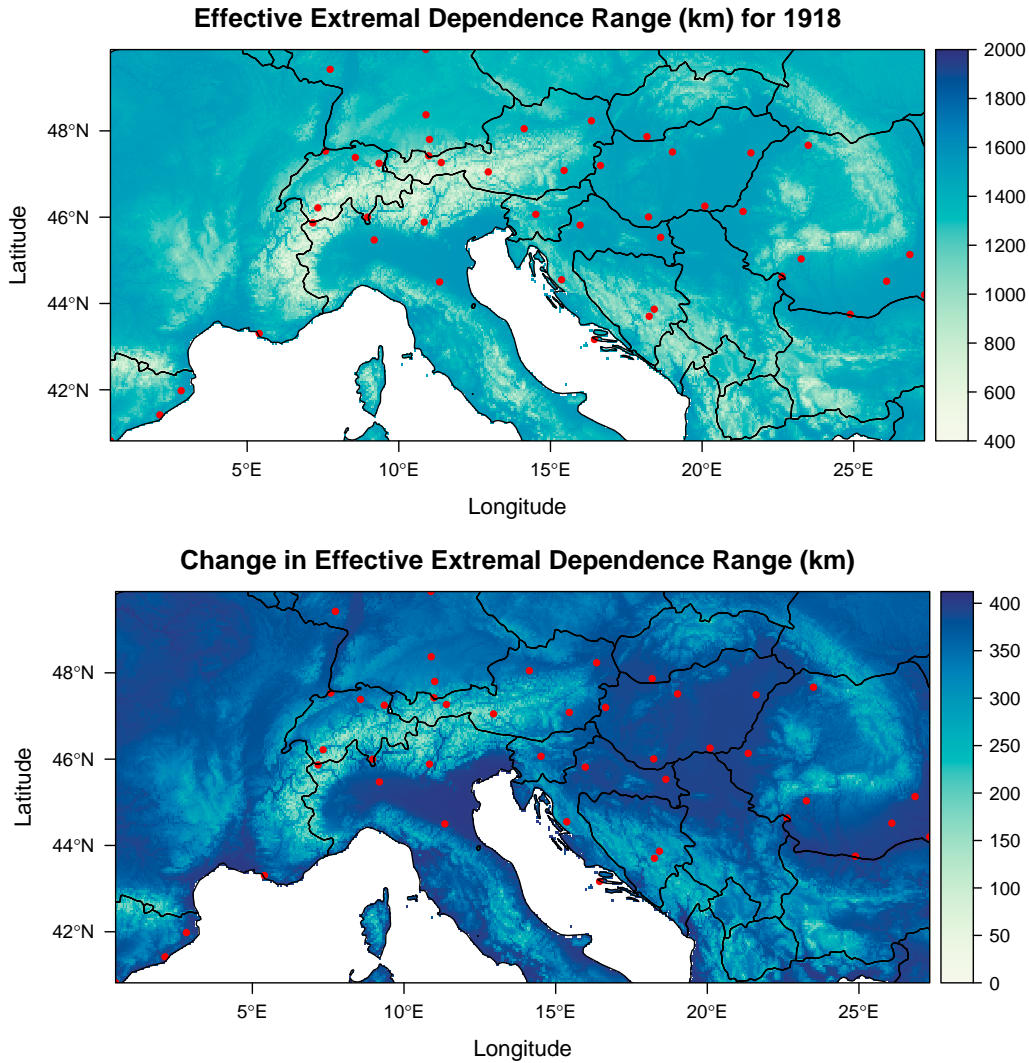
FIGURE 11. Map of the effective extremal dependence range (km) for 1918 (top), and of the difference between 2018 and 1918 (bottom), based on Model 6. The extremal dependence range is here defined as the minimum spatial distance such that \theta_2(z) = 1.95 at the level z = -1/\log(0.9) . Monitoring stations are shown as red dots.
