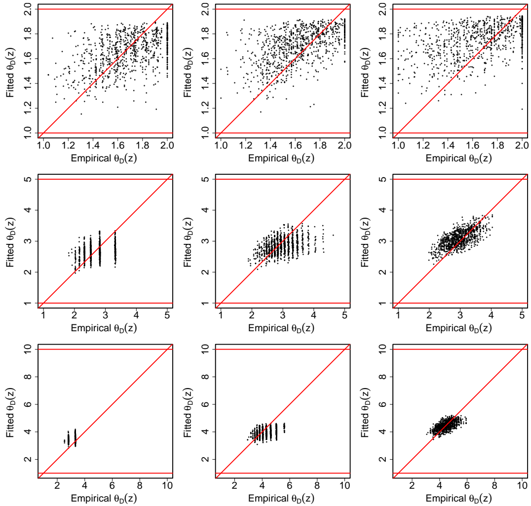
FIGURE 10. Scatterplots of empirical versus fitted extremal coefficients \theta_D(z) for Model 5 in dimensions D = 2, 5, 10 (top to bottom) for unit Fréchet quantile levels z = -1/\log(q) with q = 0.25, 0.5, 0.75 (left to right). The main diagonal indicates a perfect fit.
