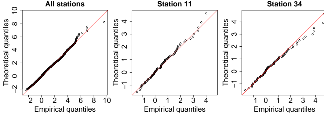
FIGURE 5. QQ-plots of maxima transformed to the standard Gumbel scale based on the fitted marginal model. Left: all stations pooled together. Middle and right: stations s_{11} and s_{34} .
