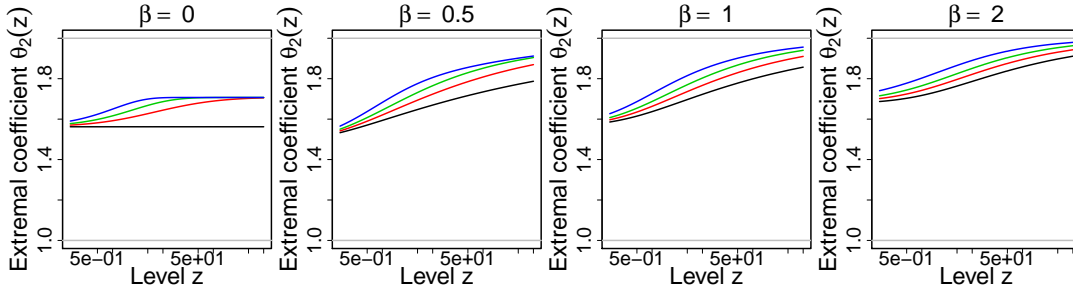
FIGURE 3. Bivariate level-dependent extremal coefficient \theta_2(z) = zV(z, z) with respect to unit Fréchet quantiles z , plotted on a logarithmic scale. Our max-id model is defined as in (3), where the mean measure \kappa of the Poisson points \{R_i\} is based on (5), here with \alpha = 1 and \beta = 0, 0.5, 1, 2 (left to right), and where the correlation function of the Gaussian processes W_i is here assumed to be \rho(\mathbf{s}_1, \mathbf{s}_2; R_i) = \exp\{-\|\mathbf{s}_1 - \mathbf{s}_2\|(1 + R_i)^\nu/\lambda\} with \lambda = 0.5 and \nu = 0 (black), \nu = 0.25 (red), \nu = 0.5 (green), \nu = 1 (blue). The distance \|\mathbf{s}_1 - \mathbf{s}_2\| is here set to 0.5. The horizontal grey lines represent the lower and upper bounds of 1 and 2, respectively.
