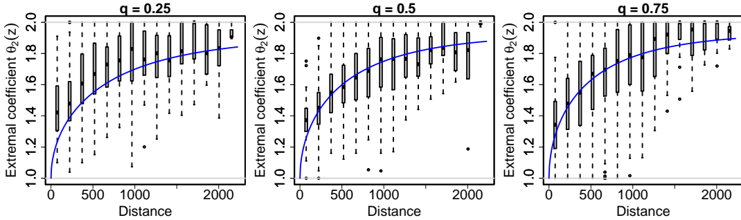
FIGURE 9. Boxplots of empirical bivariate extremal coefficients \theta_2(z) computed for all pairs of sites within 15 equally spaced distance classes, and theoretical curve (blue) based on the fitted Model 5 plotted with respect to spatial distance, for unit Fréchet quantile levels z = -1/\log(q) with q = 0.25, 0.5 and 0.75 (left to right).
