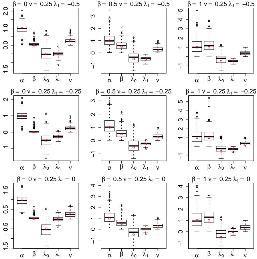
FIGURE 4. Boxplots of estimated parameters for the simulation study described in §4.3. Each panel corresponds to a different simulation scenario with \lambda_1 = -0.5, -0.25, 0 (top to bottom) and \beta = 0, 0.5, 1 (left to right) (see details in the text), and shows boxplots for each of the 5 parameters based on 200 experiments. Red dots indicate the true values.
