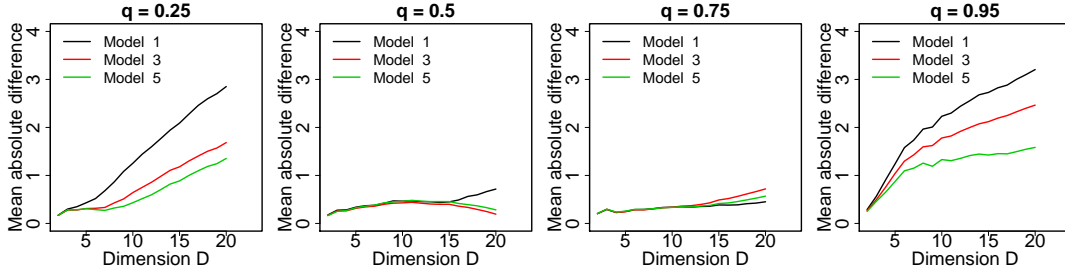
FIGURE 8. Mean absolute difference between empirical and fitted extremal coefficients \theta_D(z) , plotted with respect to dimension D = 2-20 , for Models 1 (black), 3 (red), and 5 (green), at unit Fréchet quantile levels z = -1/\log(q) with q = 0.25, 0.5, 0.75 and 0.95 (left to right).
